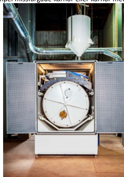
Figuren visar BoMills TriQ-sorterare
